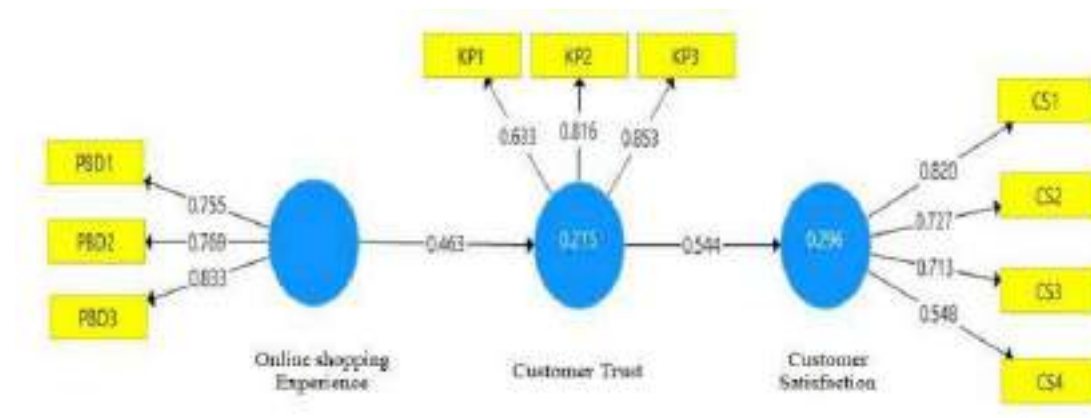
Figure 2. Path Diagram Outer Model
